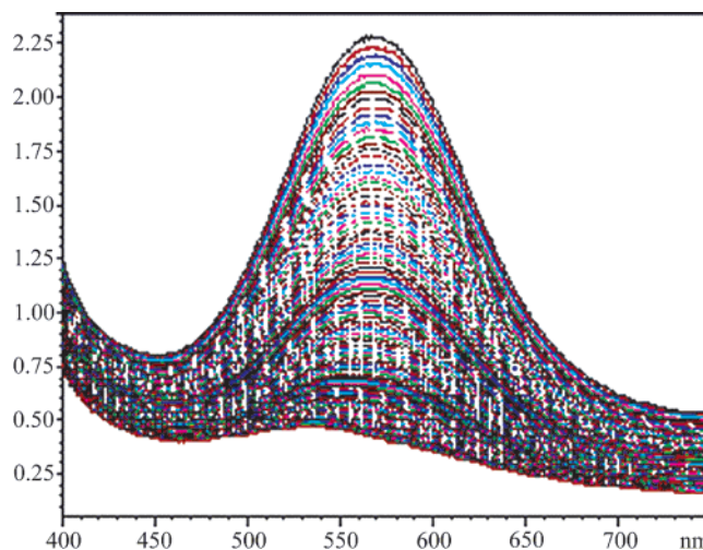
Figure 8. Representative UV-vis spectrum for the cyclopropanation of styrene (100 equiv) by [Me_2NN]Cu=CPh_2 ( 8 ) (dioxane, 30.2 °C).
