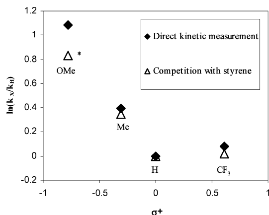
Figure 10. Hammett plot of cyclopropanation of p -substituted styrenes. (* denotes estimated value due to overlapping GC peaks in competition experiment.)
