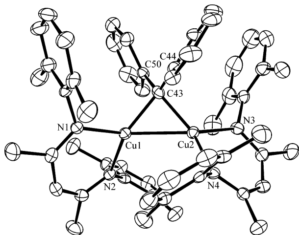
Figure 2. ORTEP diagram of the solid-state structure of \{[\text{Me}_2\text{NN}]\text{Cu}\}_2(\mu\text{-CPh}_2) ( 3 ) (all H atoms omitted). Selected bond distances (angstroms), angles (deg), and twist angles between planes (deg): Cu1–C43 1.922(4), Cu2–C43 1.930(4), Cu1–Cu2 2.4635(7), Cu1–N1 1.965(3), Cu1–N2 1.955(3), Cu2–N3 1.970(3), Cu2–N4 1.978(3), Cu1–C43–Cu2 79.51(14), N1–Cu1–N2 96.11(13), N3–Cu2–N4 95.85(12), C44–C43–C50 115.0(3), N1–Cu1–N2/C44–C43–C50 89.1, N3–Cu2–N4/C44–C43–C50 83.1.
