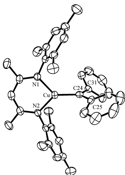
Figure 7. ORTEP diagram of the solid-state structure of [Me_3NN]Cu=CPh_2 ( 8 ) (all H atoms omitted). Selected bond distances (angstroms), angles (deg), and twist angles between planes (deg): Cu–C24 1.834(3), Cu–N1 1.906(3), Cu–N2 1.922(3), N1–Cu–N2 96.10(12), C25–C24–C31 117.3(3), N1–Cu–N2/C25–C24–C31 89.0.
