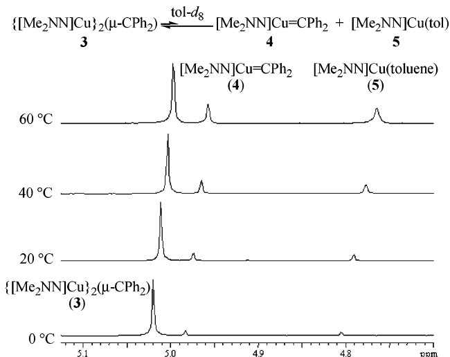
Scheme 1. Variable Temperature ^1\text{H} NMR Spectra (300 MHz) of the \beta -Diketiminato Backbone C–H Region of 3 in Toluene- d_8
