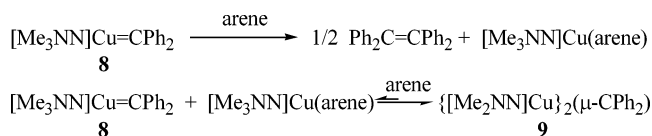
Scheme 3. Formation of Dicopper Carbene 9 via Decomposition of 8 in Arene Solvents
