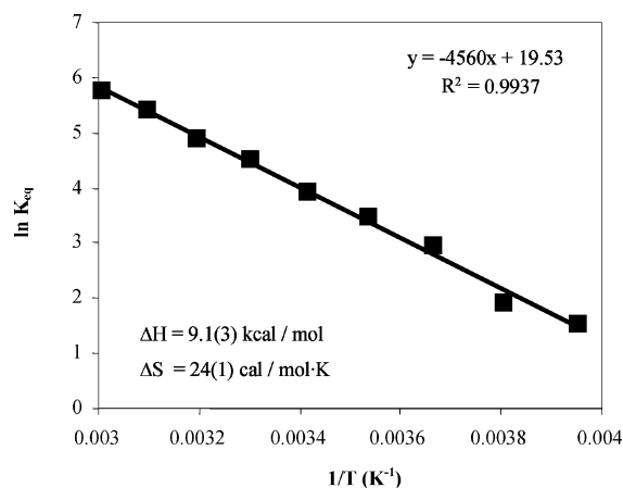
Figure 3. van't Hoff plot for the dissociation of a [\text{Me}_2\text{NN}]\text{Cu} fragment from 3 in toluene- d_8 .
