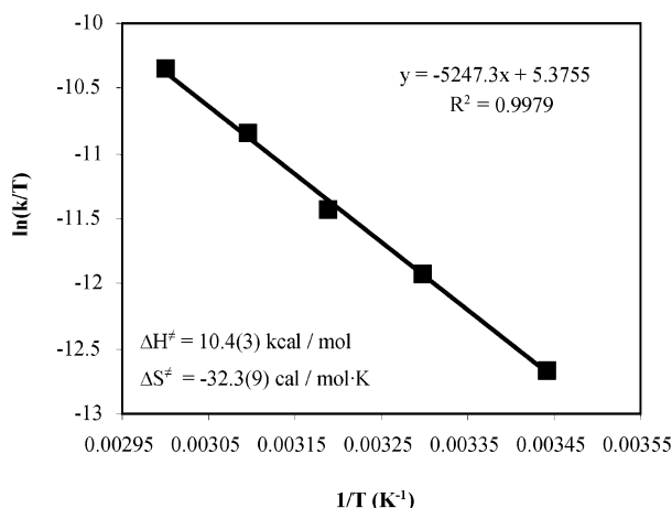
Figure 9. Eyring plot for the cyclopropanation of styrene by 8 in dioxane over the temperature range 17.5–60.2 °C.
