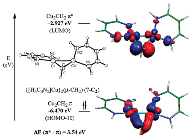
Figure 6. Cu-carbene orbital interactions in C_2 symmetric \{[H_5C_3N_2]Cu\}_2(\mu-CH_2) ( 7-C 2 ).
