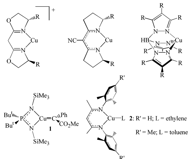
Figure 1. Supporting ligands in copper cyclopropanation catalysts.
