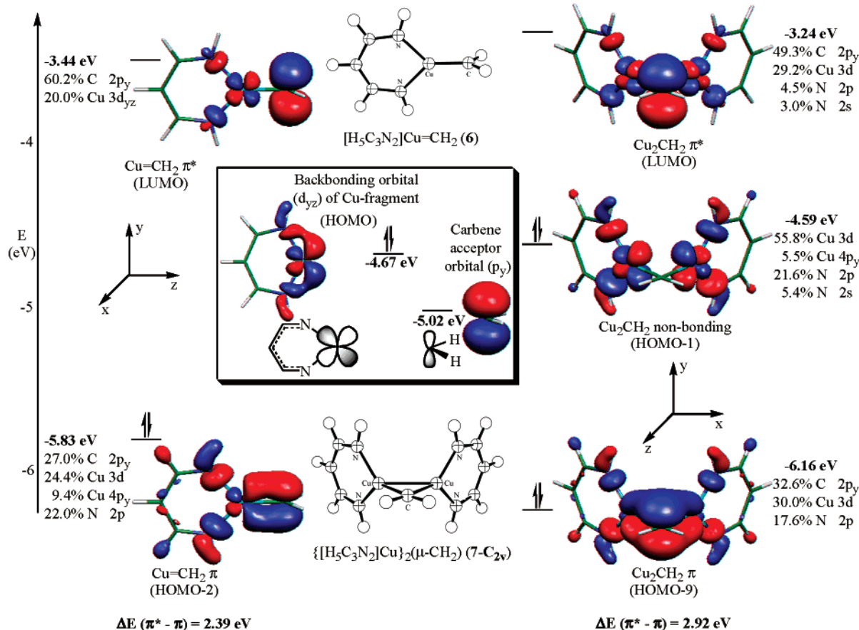
Figure 5. Correlation diagram illustrating Cu–C \pi -interactions in \text{C}_{2v} symmetric monocarbene 6 (left) and dicopper carbene 7- \text{C}_{2v} (right).
