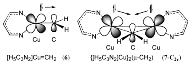
Figure 4. \pi -Back-bonding interactions in \text{C}_{2v} symmetric copper carbenes.
